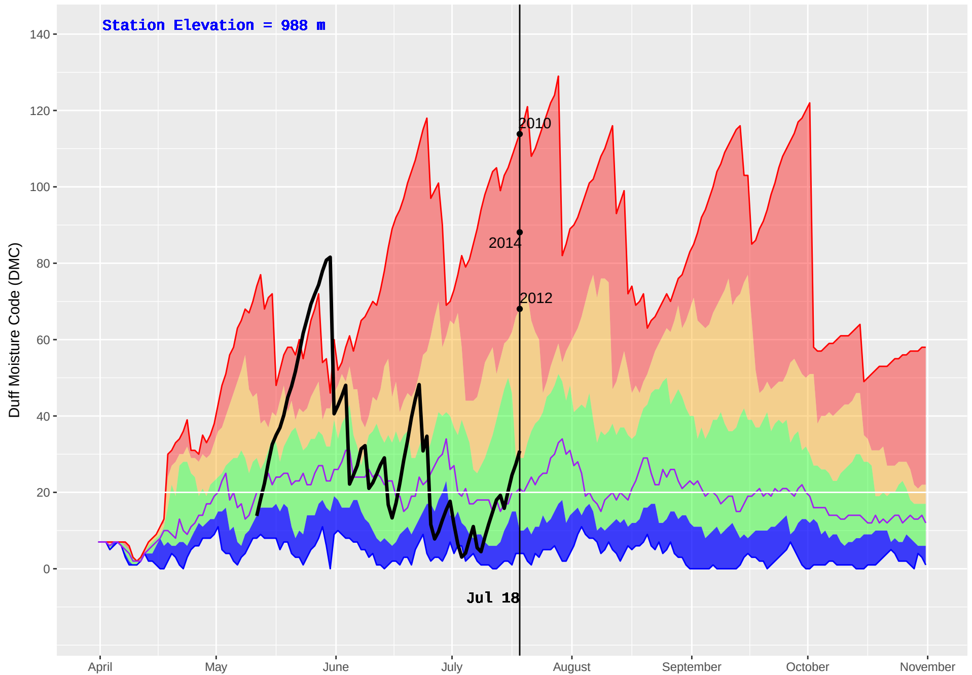
NOEL (437) : Historical (1993–2016) and Current (2018) Daily Duff Moisture Code (DMC)
