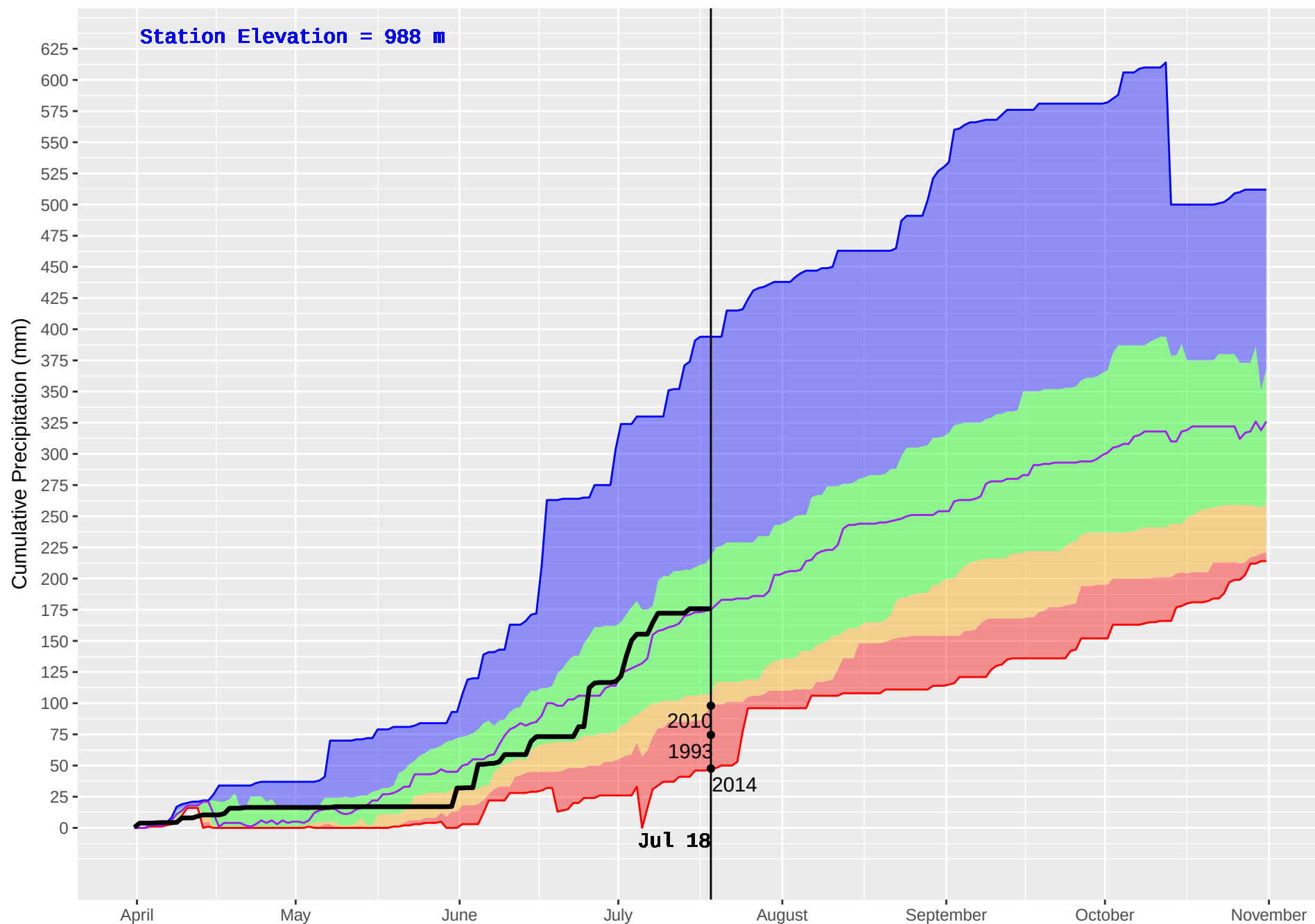
NOEL (437) : Historical (1993–2016) and Current (2018) Daily Cumulative Precipitation
