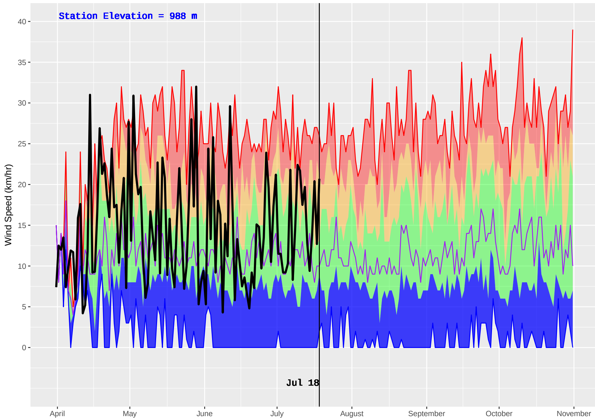
NOEL (437) : Historical (1993–2016) and Current (2018) Daily Wind Speed
