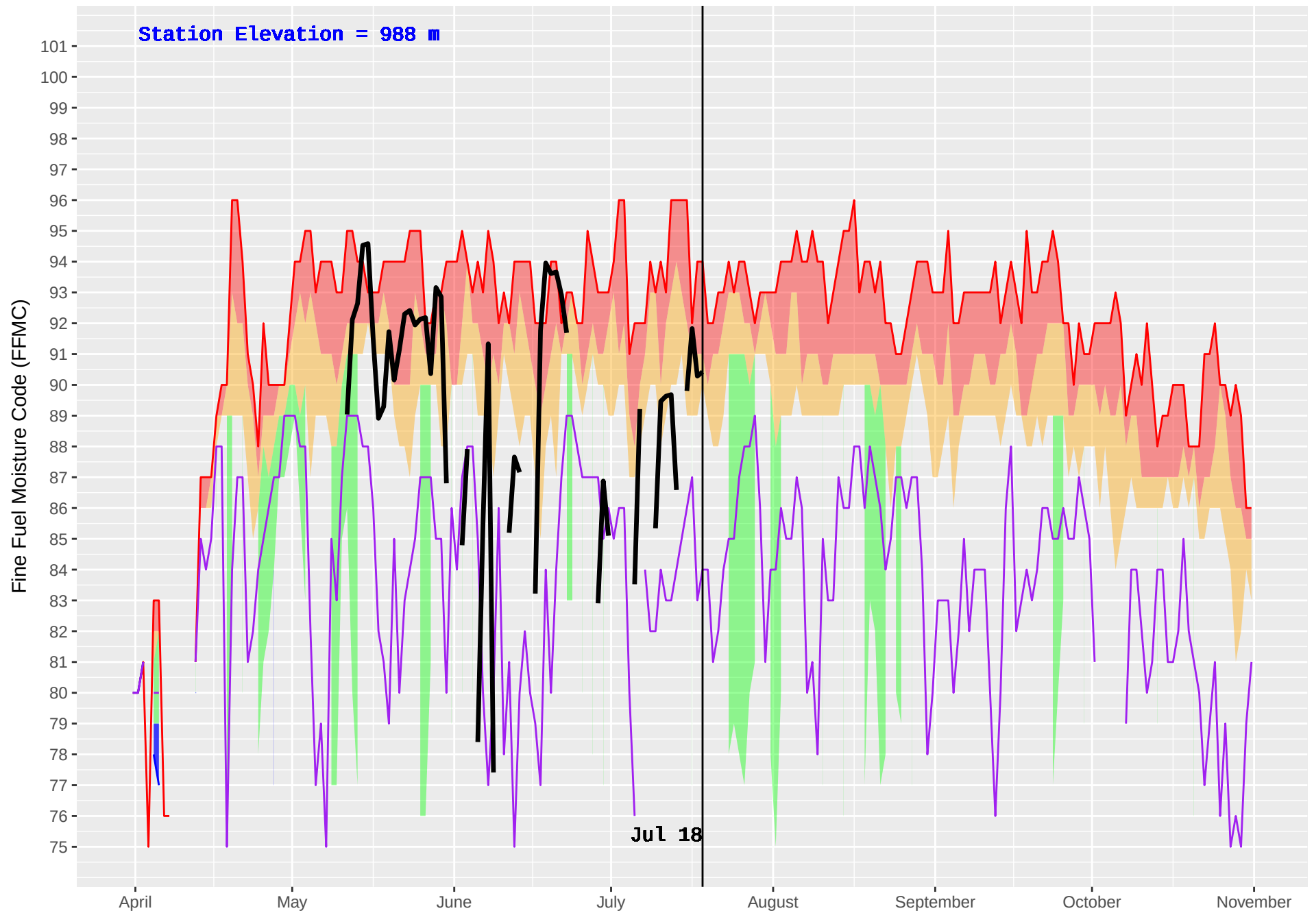
NOEL (437) : Historical (1993–2016) and Current (2018) Daily Fine Fuel Moisture Code (FFMC)
