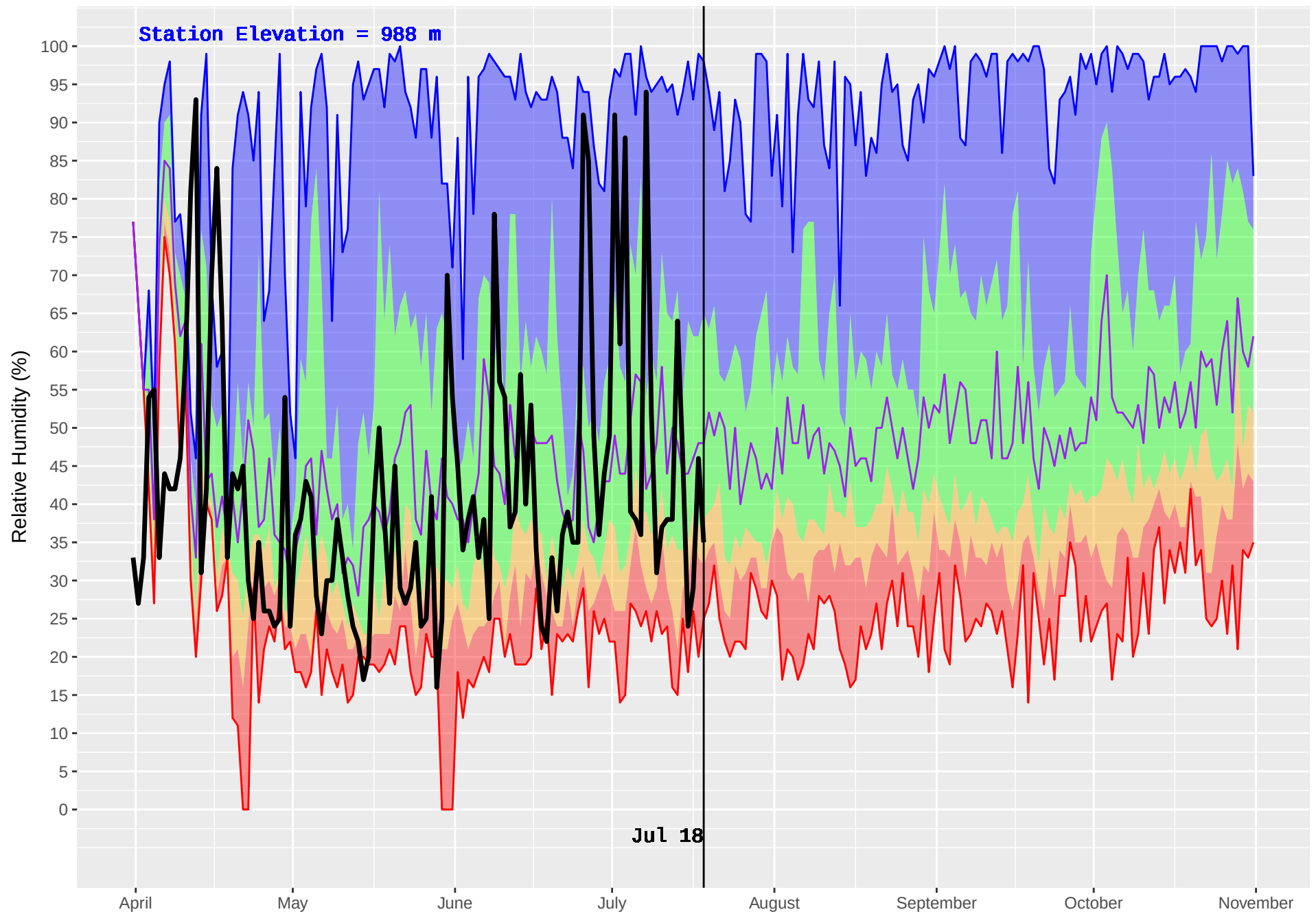
NOEL (437) : Historical (1993–2016) and Current (2018) Daily Relative Humidity
